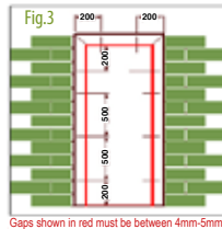
Gaps shown in red must be between 4mm-5mm
